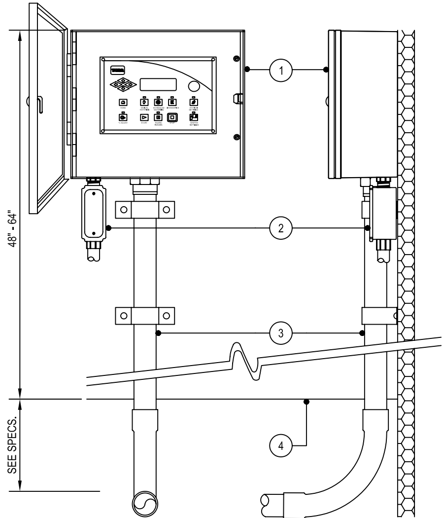
FRONT SECTION/ELEVATION
